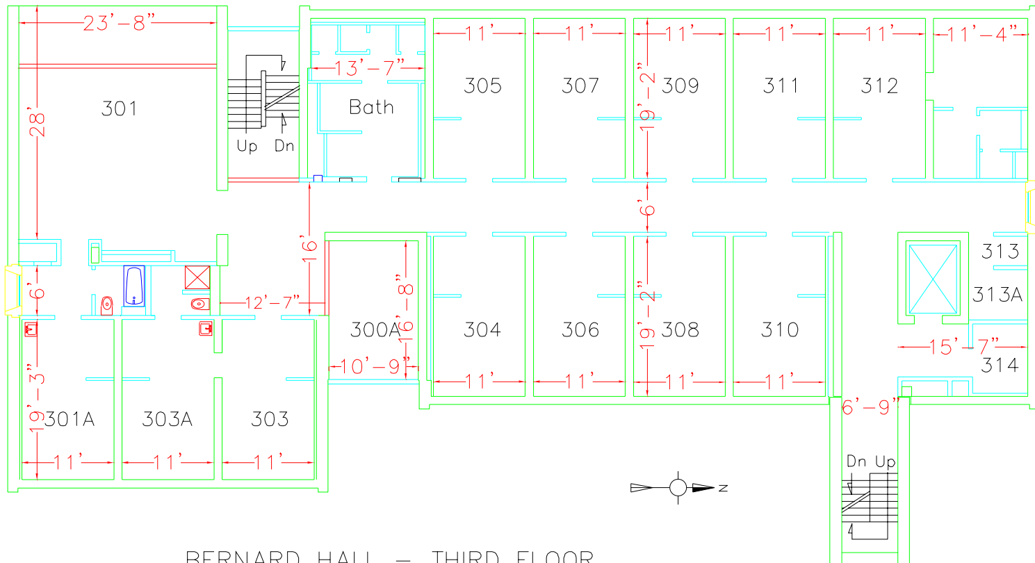
BERNARD HALL – THIRD FLOOR Scale: 1/16" = 1'-0"
