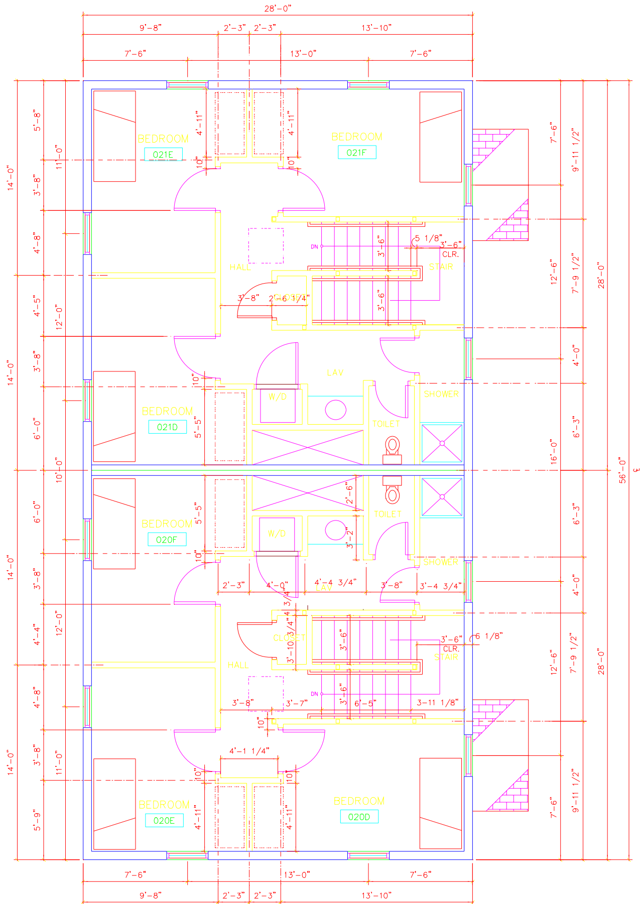
TYPICAL VINCENT COURT LEVEL 3
