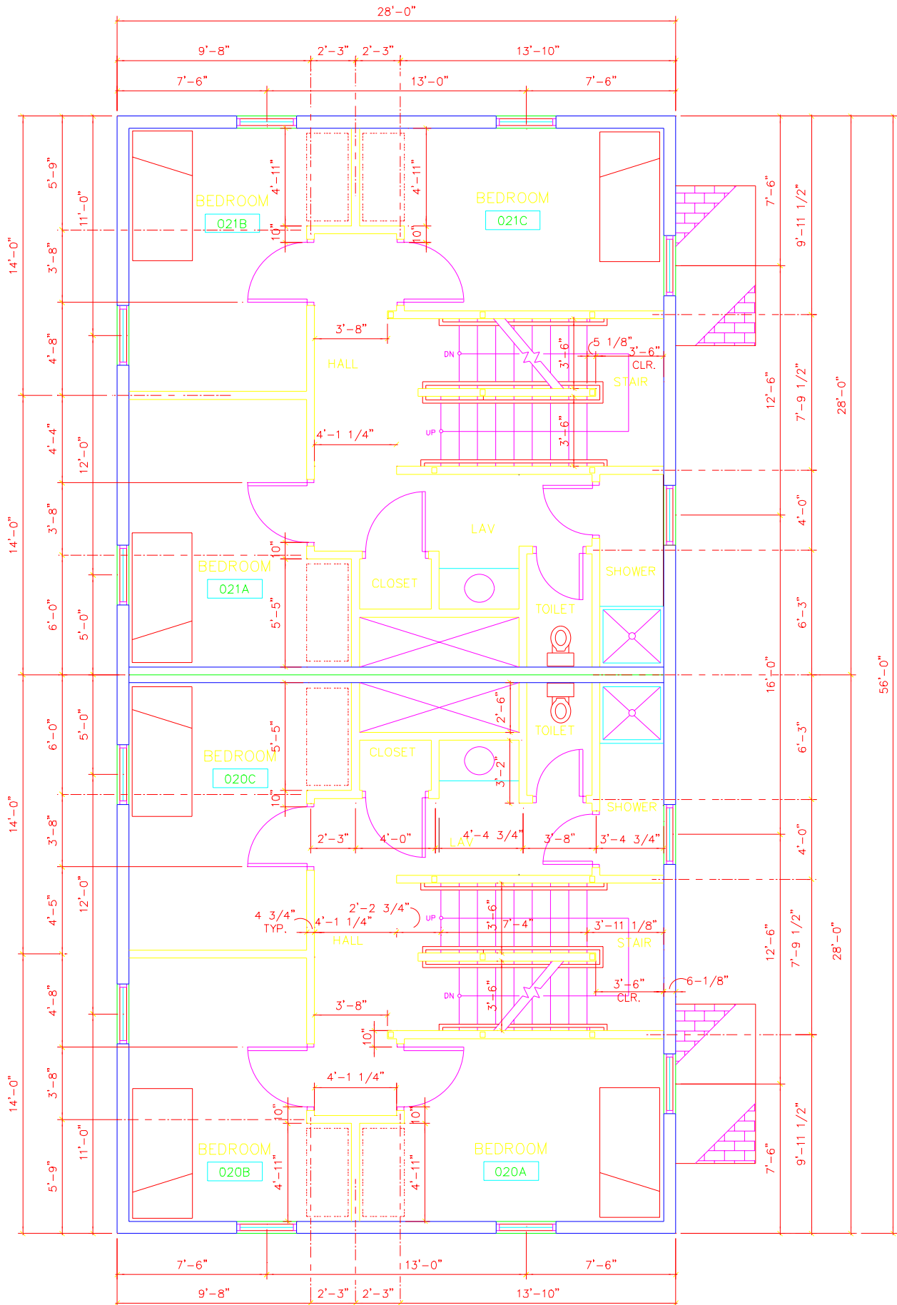
TYPICAL VINCENT COURT LEVEL 2
