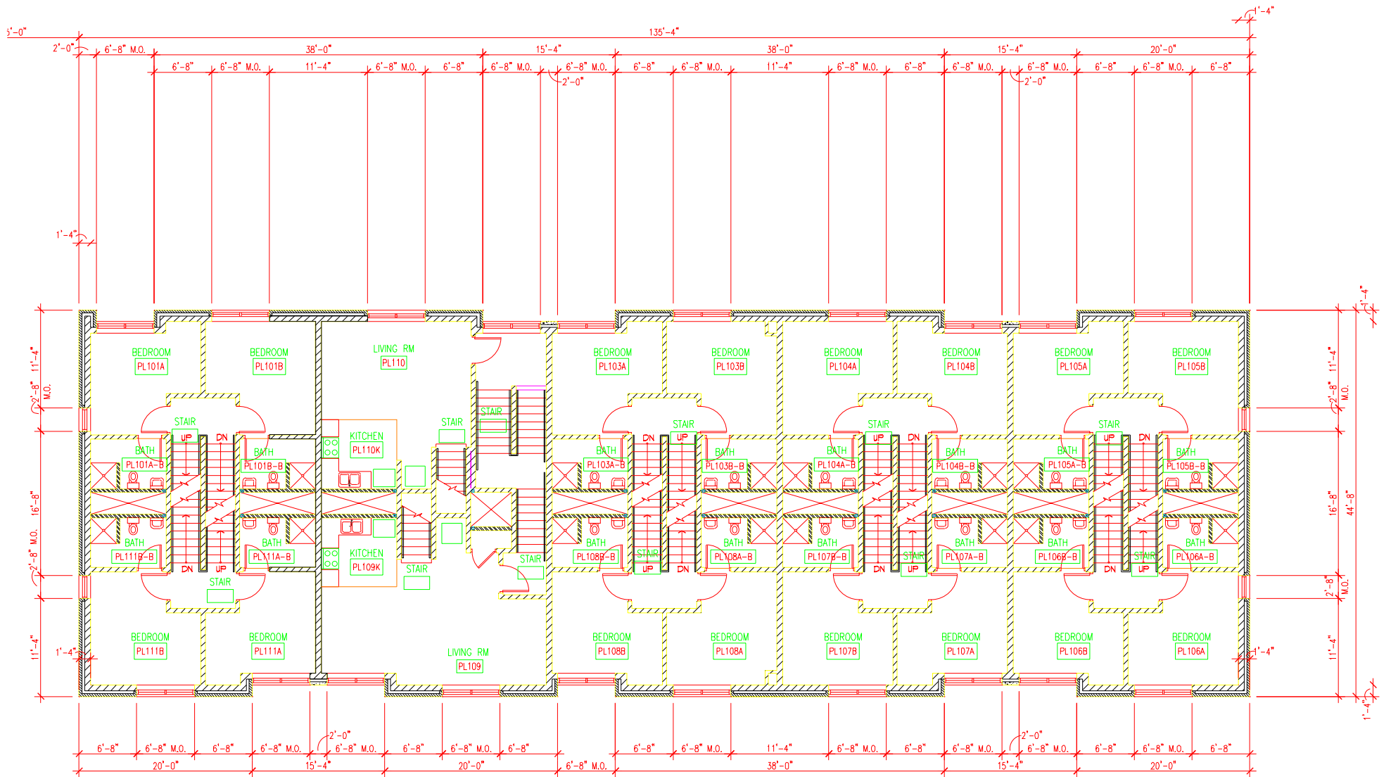
Saint Placid House—2nd Floor
