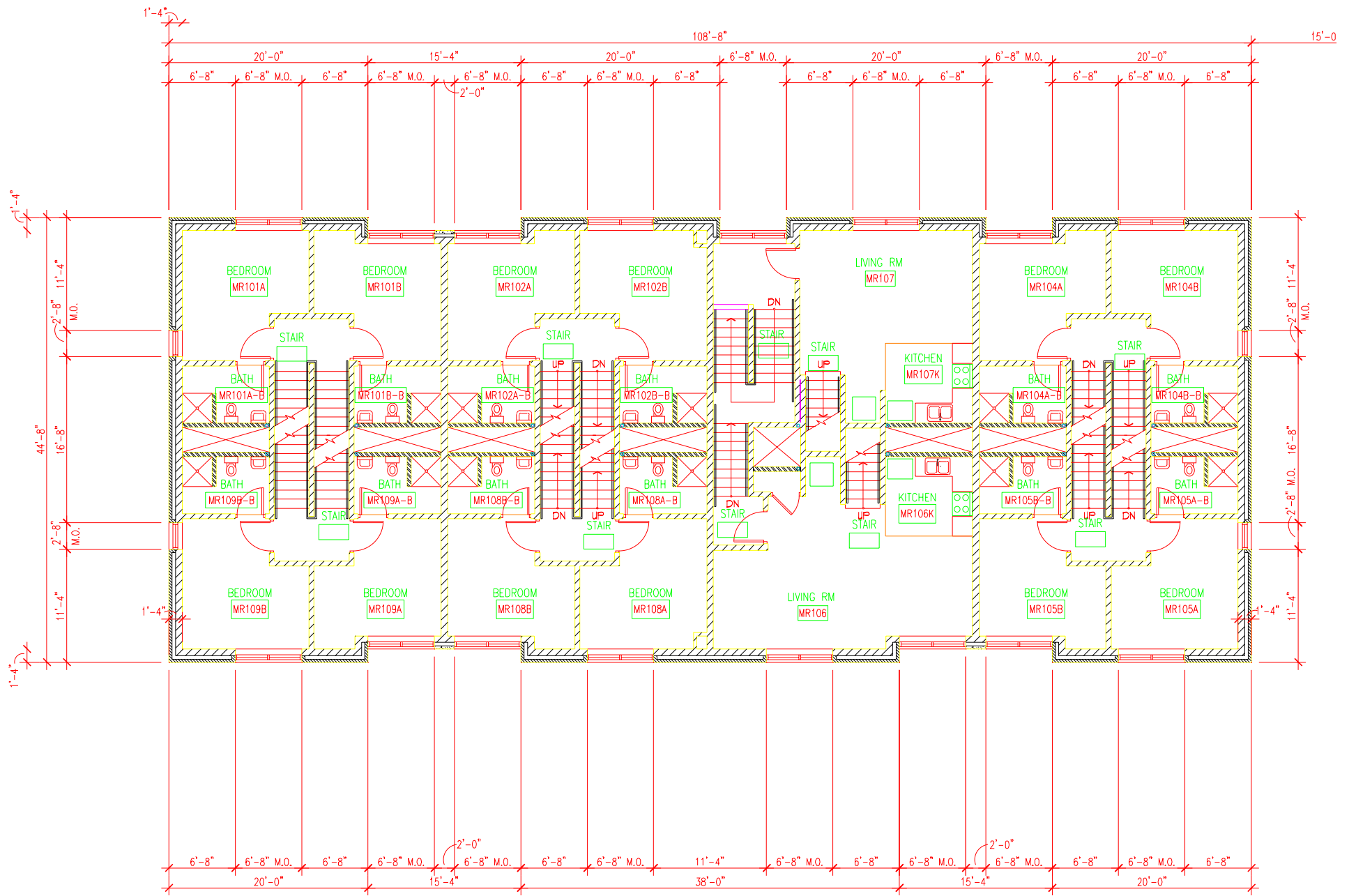
Saint Mauer House—2nd Floor
